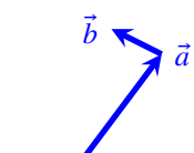
Figure 2.5 Visualisation of “head to tail” addition of \vec{a} and \vec{b} .
