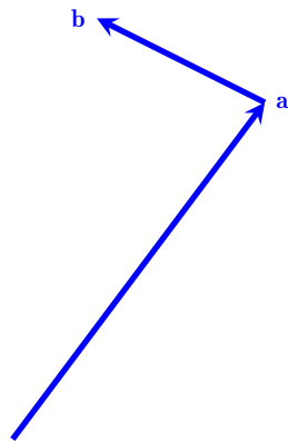
Fig. 2.5 Visualization of "head to tail" addition of \mathbf{a} and \mathbf{b} .
