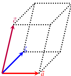
Figure 2.18 Figure of triple vector multiplication.
