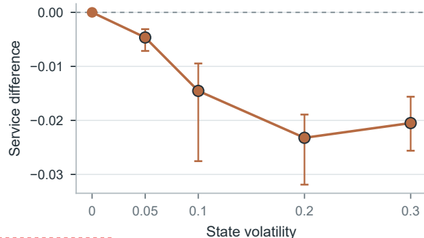
d Stability: immediate service cost Wilcoxon-adjusted P < 0.05
