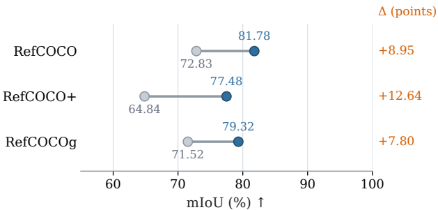
(a) mIoU
