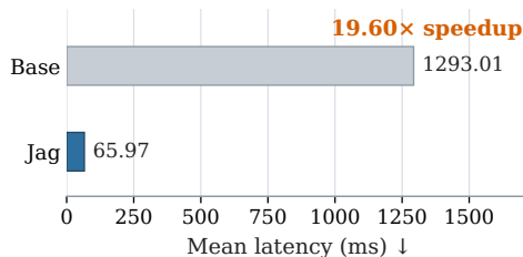
(c) Prediction latency
