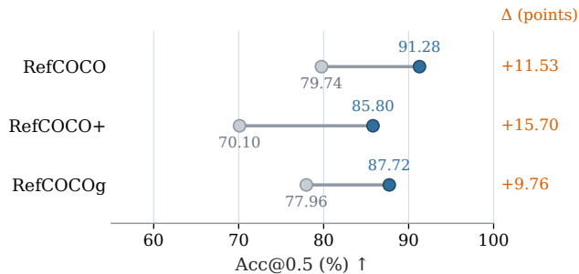
(b) Acc@0.5
