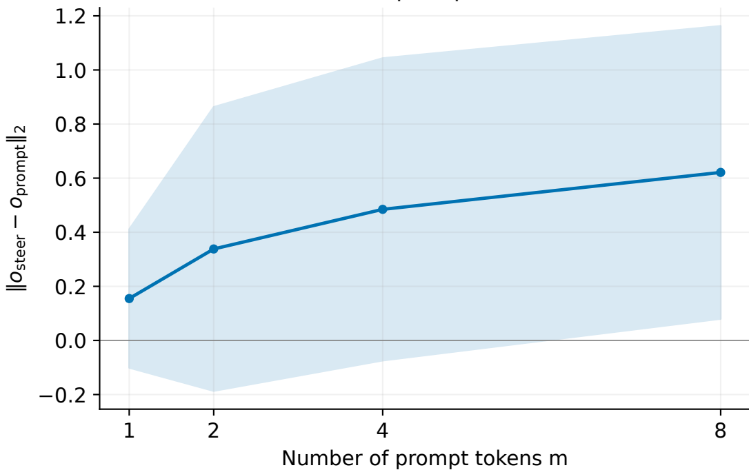
Fixed single-token steering ( k = 1 ) Qwen3-4B / 400 prompts · mean \pm std
