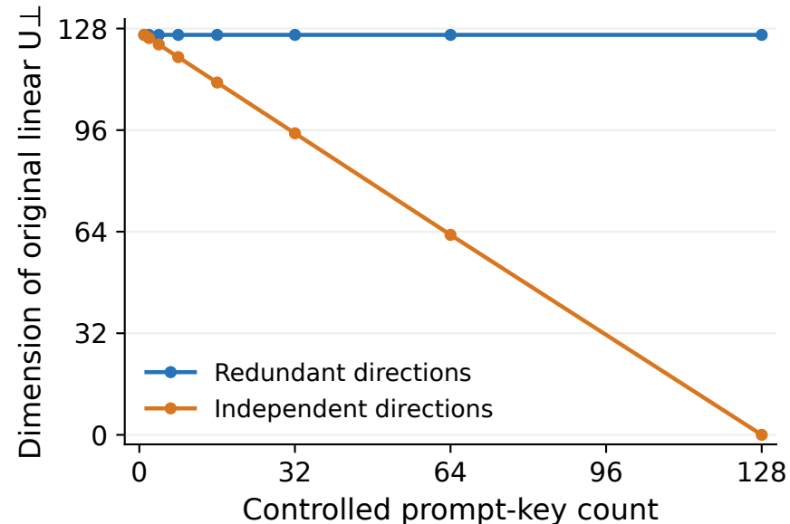
Linear key-space diagnostic; fixed value-null direction within each example/head
