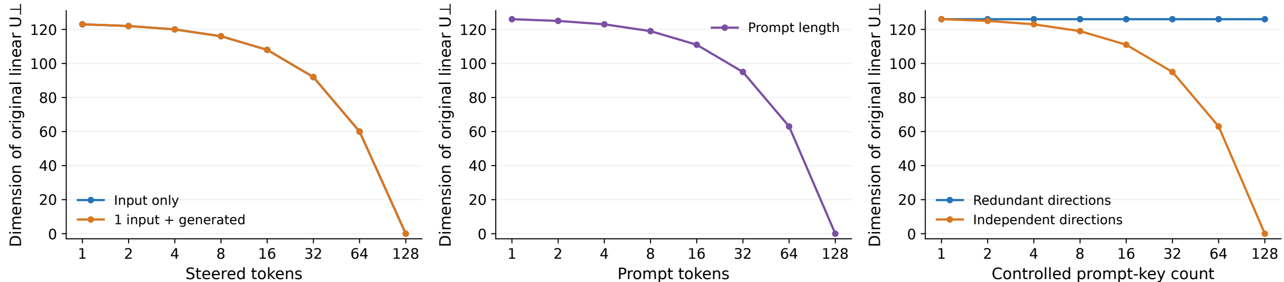
Linear key-space diagnostic; fixed value-null direction within each example/head
