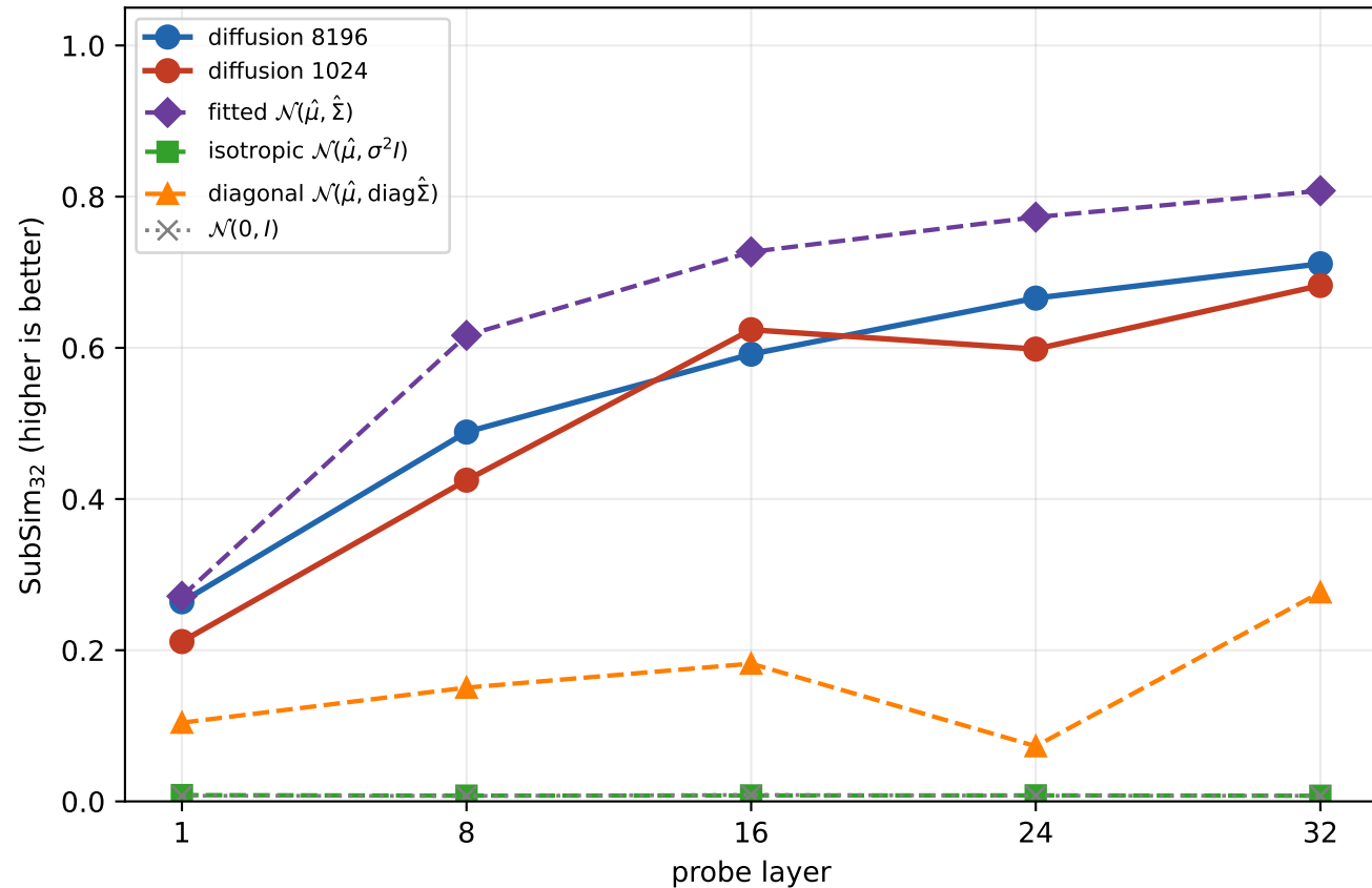
Top-32 principal subspace alignment
