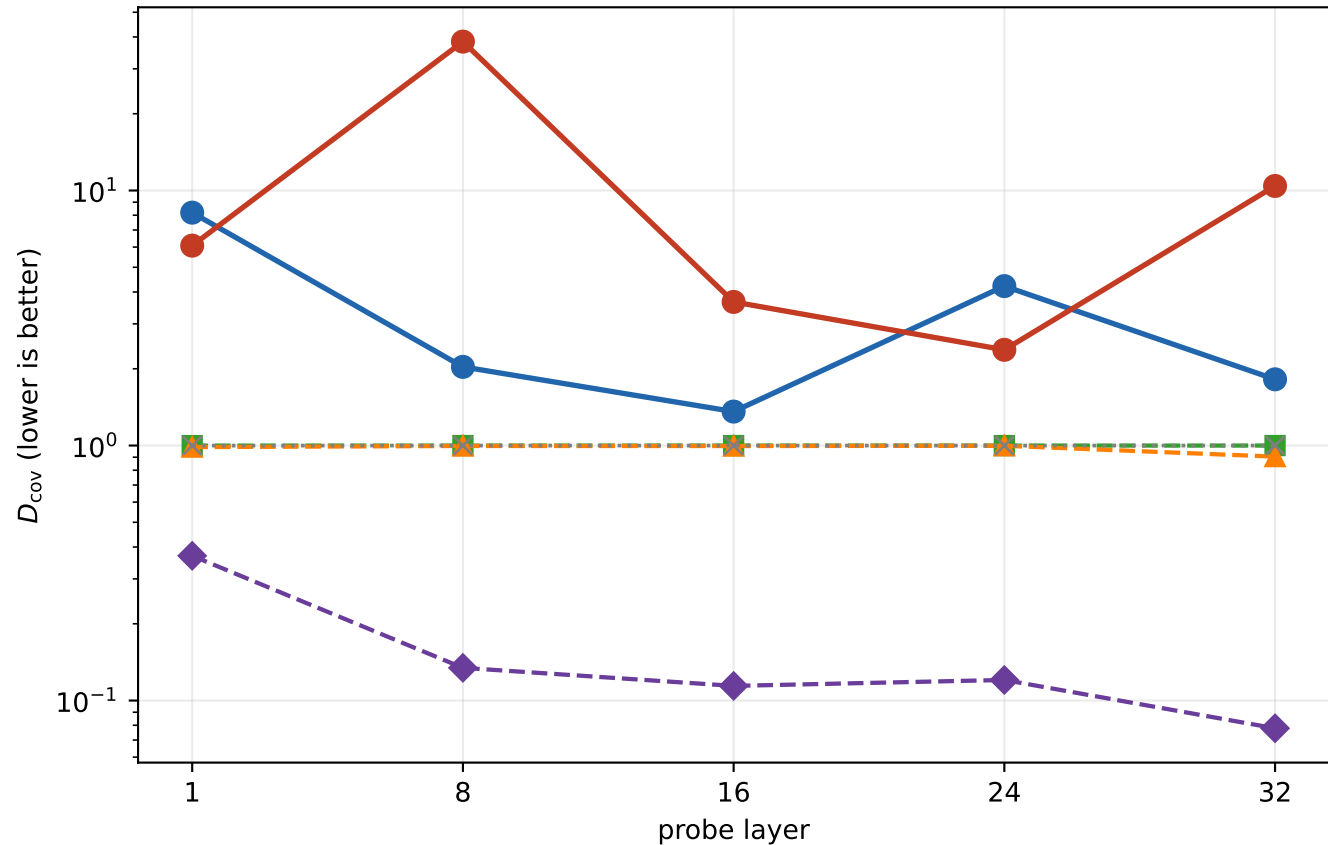
Full 4096-d covariance discrepancy
