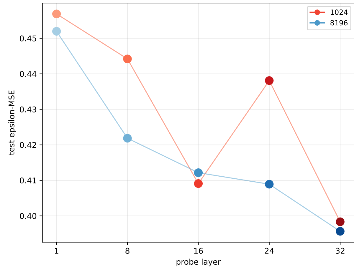
Test loss at best checkpoint
