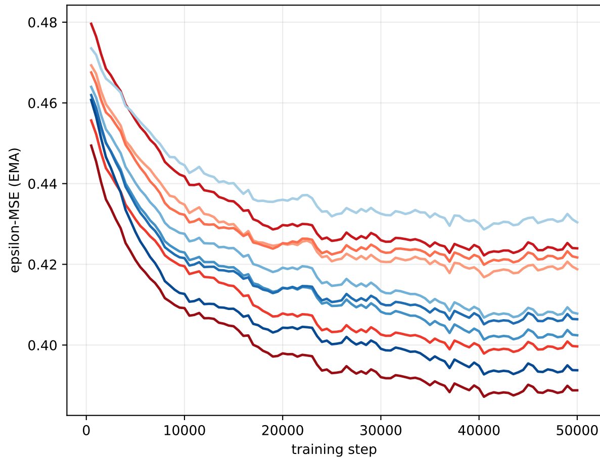
Validation loss
