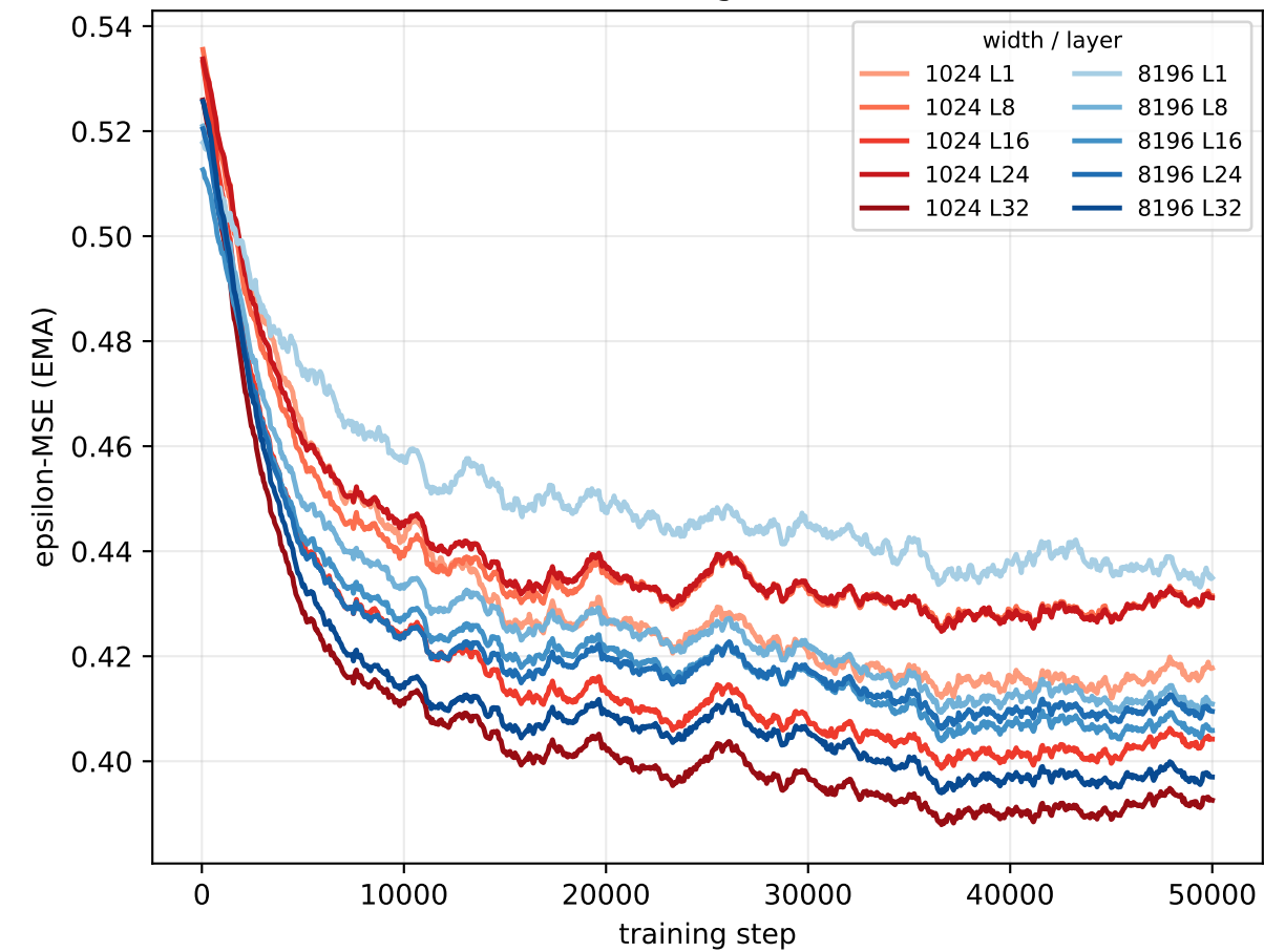
Training loss
