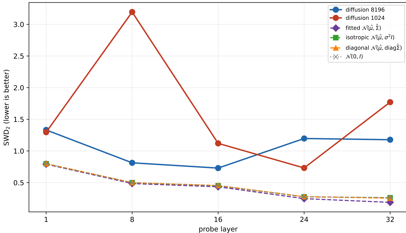
Sliced Wasserstein-2 vs real test states
