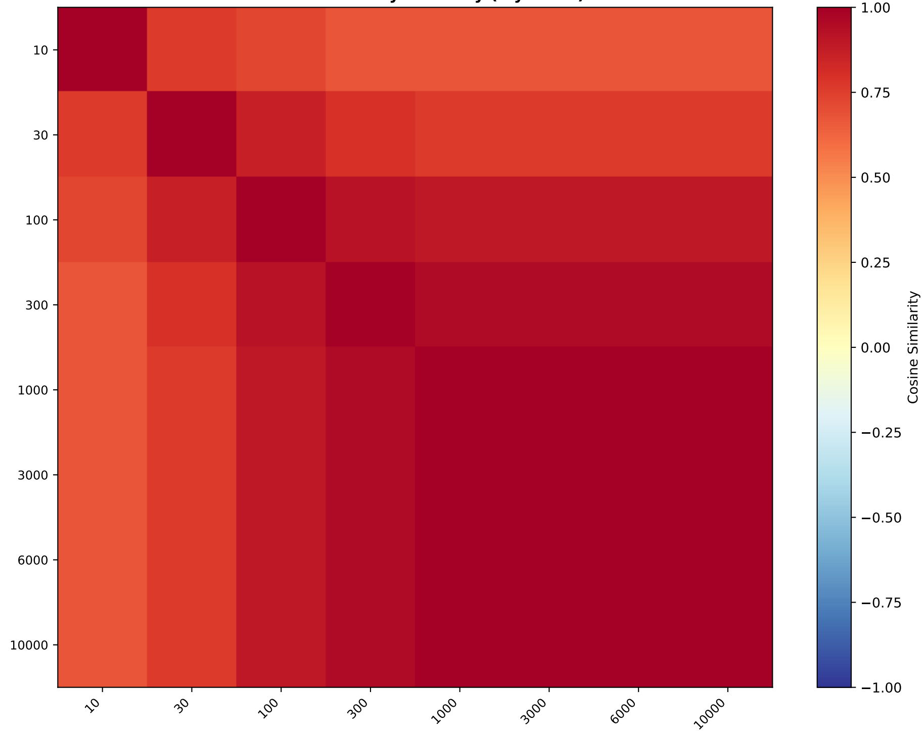
Cosine Similarity: honesty (layer 0.8)
