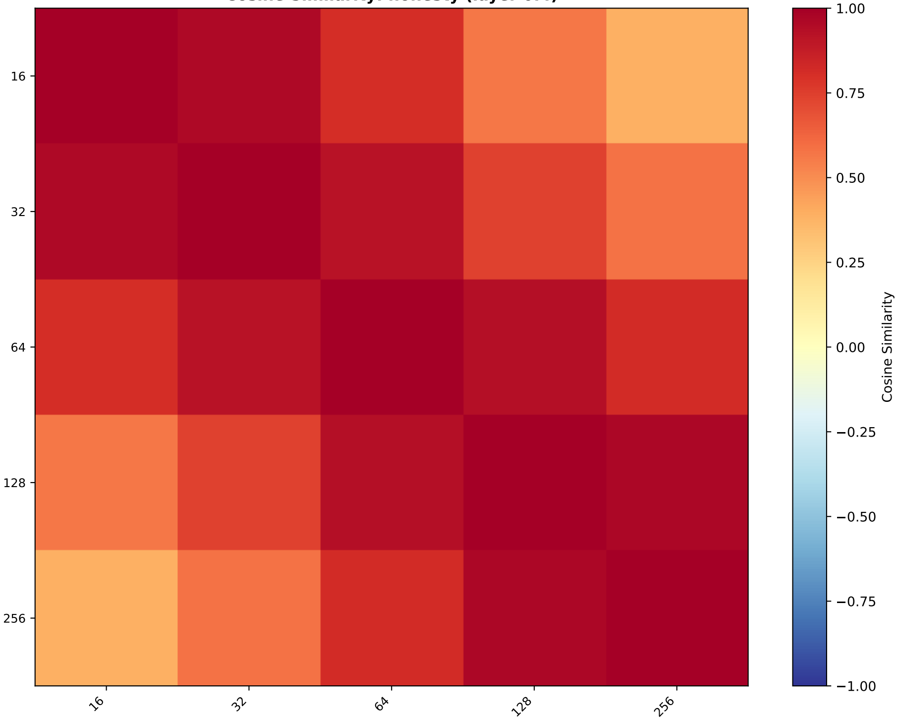
Cosine Similarity: honesty (layer 0.4)
