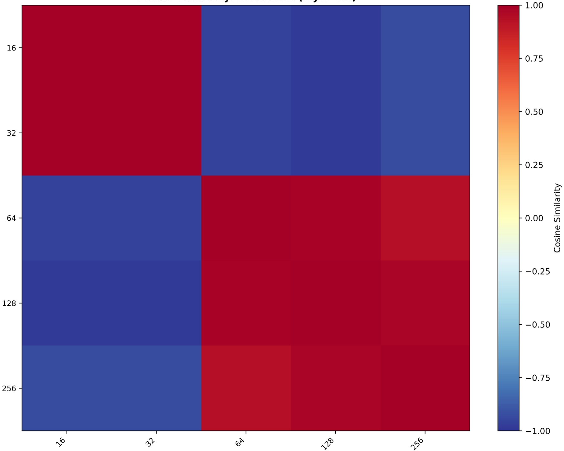
Cosine Similarity: sentiment (layer 0.6)
