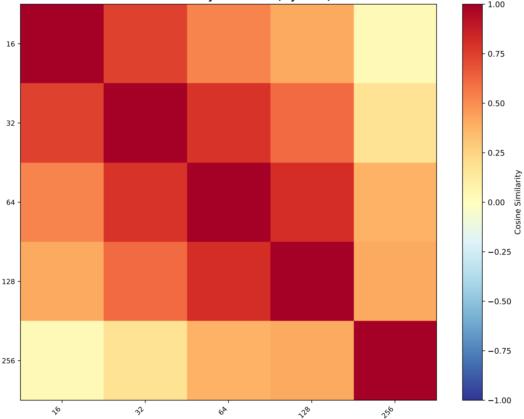
Cosine Similarity: sentiment (layer 0.7)
