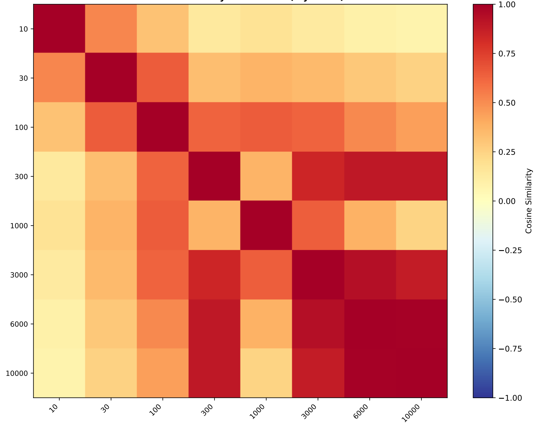
Cosine Similarity: sentiment (layer 0.8)
