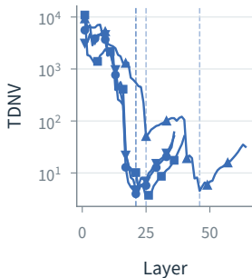
(a) Qwen3
