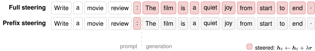
Figure 1 Teaser. Full steering shifts the hidden state at every generated position; Prefix Steering shifts it only over a short span starting at the final prompt token, and generation continues from the context this creates.
