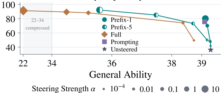
(a) Safety–capability trade-off
