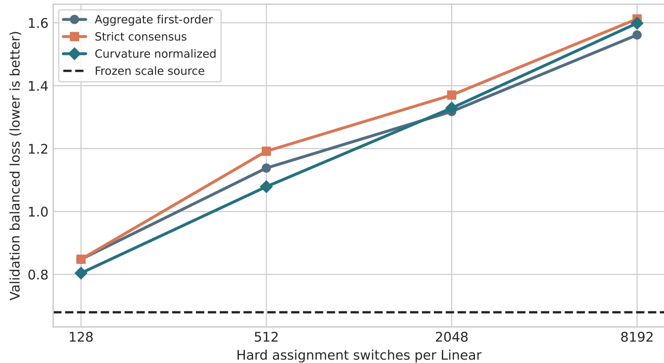
Local curvature improves ranking, but every hard set loses to source
