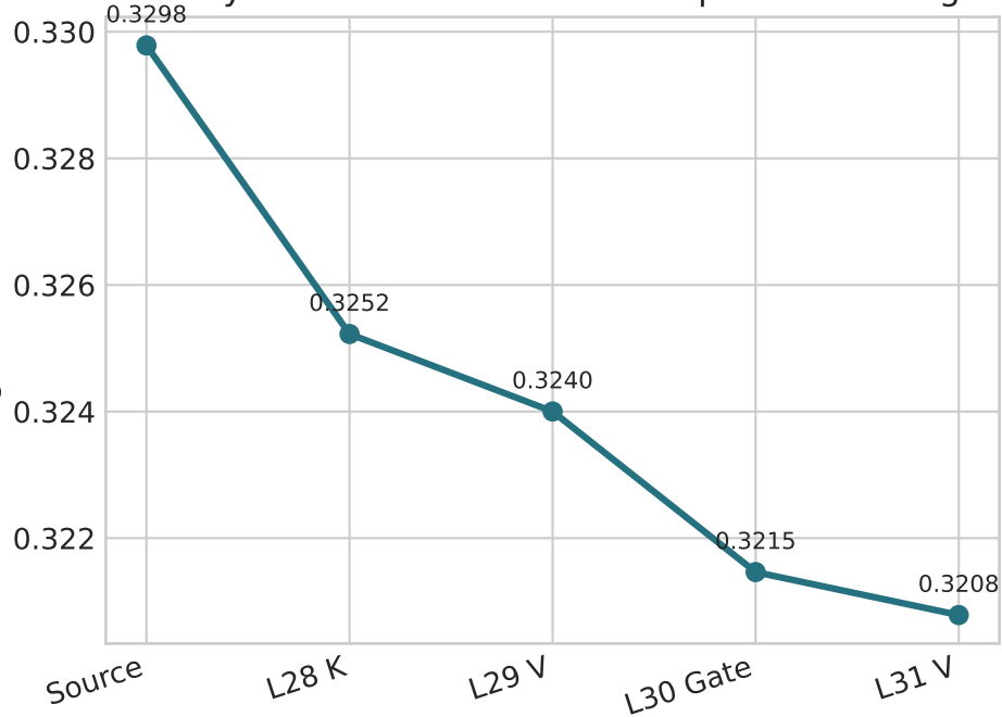
Every conditional coordinate improves training
