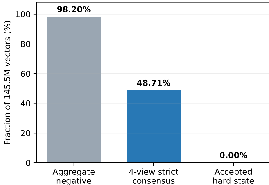
Consensus filters conflict, not curvature
