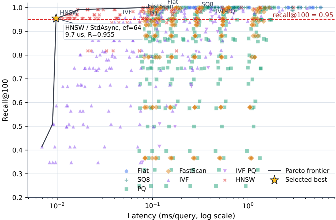
Recall-Latency Frontier Under the Target Constraint
