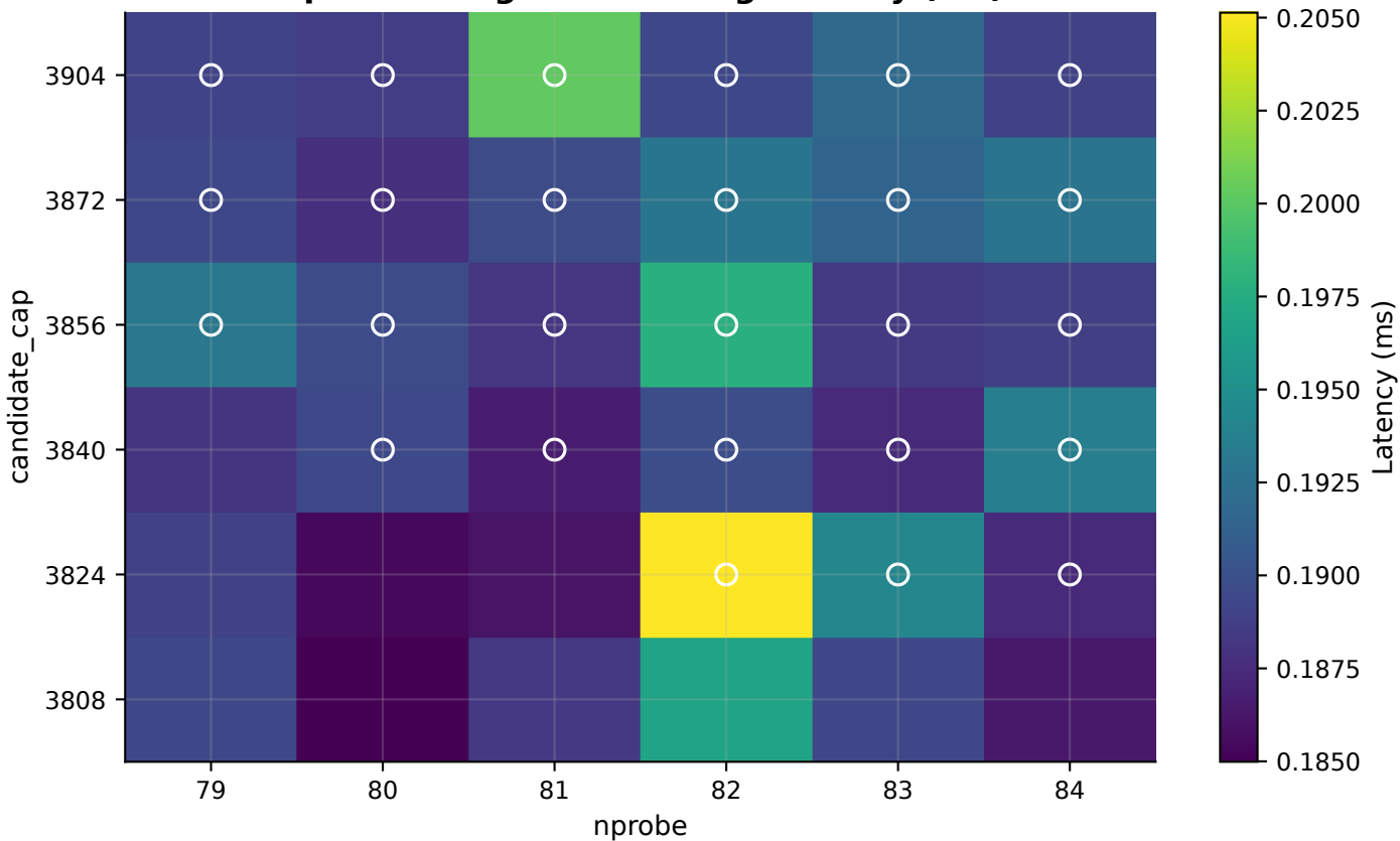
OpenMP Target IVF Tuning Latency (ms)
