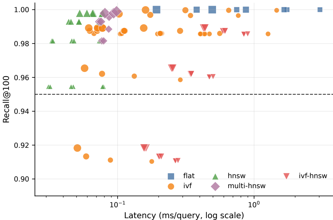
Recall-latency frontier on full DEEP100K
