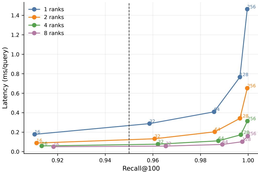
IVF nprobe trade-off under MPI data partitioning
