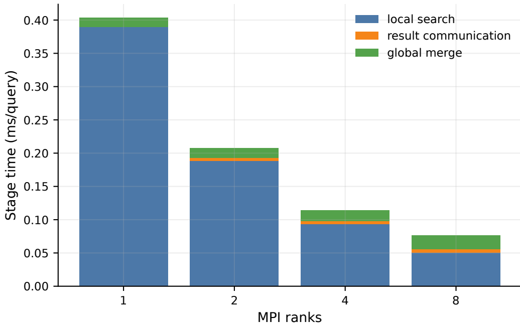
IVF stage breakdown at nprobe=64
