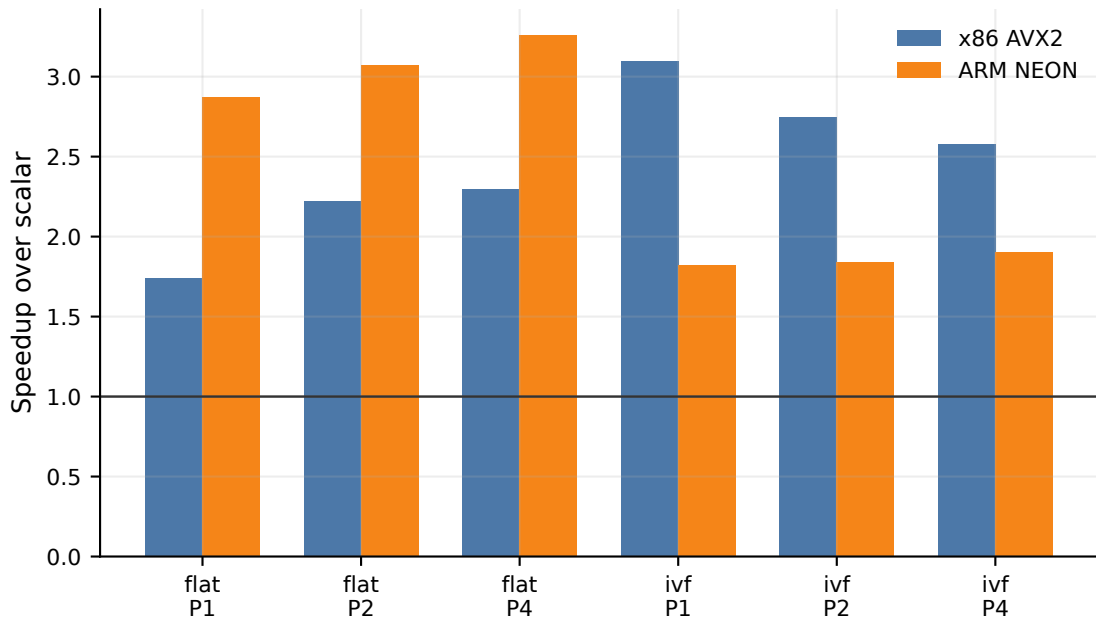
SIMD contribution inside MPI ranks
