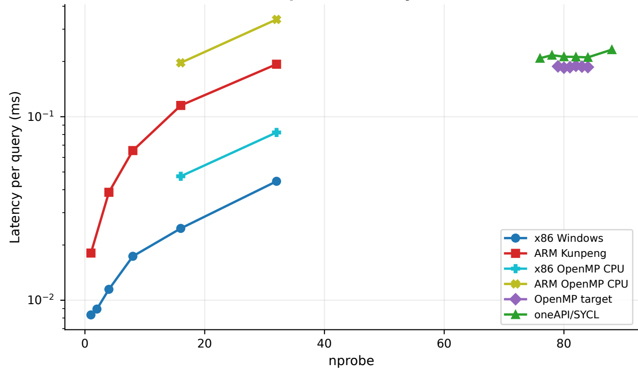
IVF nprobe Latency Cost
