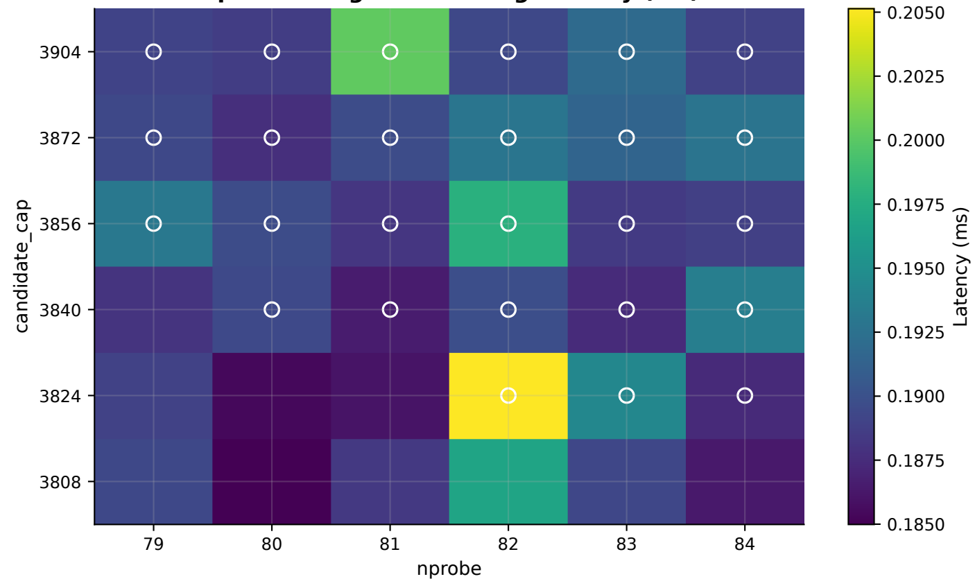
OpenMP Target IVF Tuning Latency (ms)
