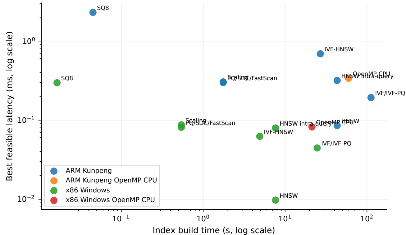
Index Build Cost vs Selected Query Latency
