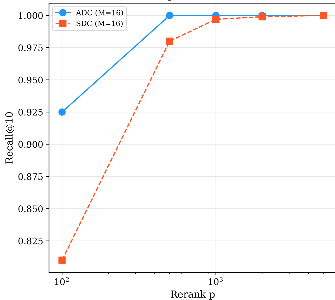
Recall Comparison (M=16, x86)
