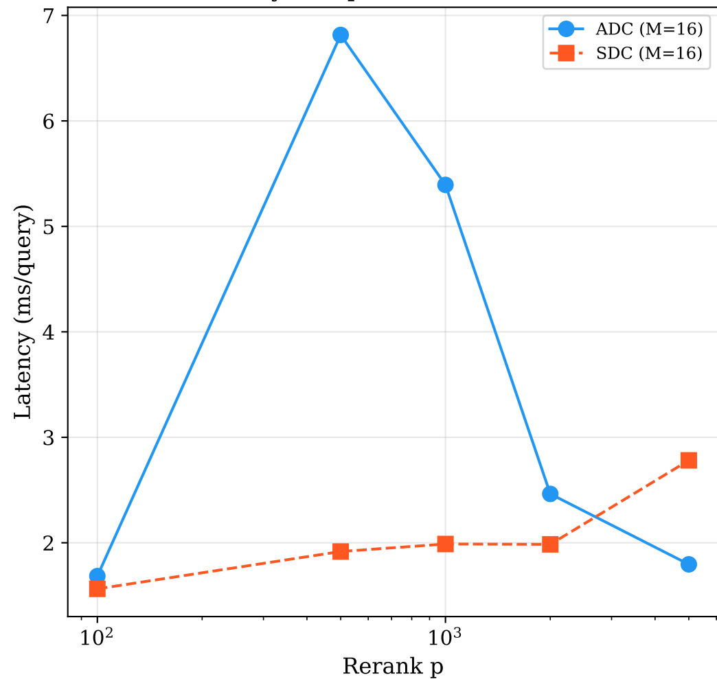
Latency Comparison (M=16, x86)
