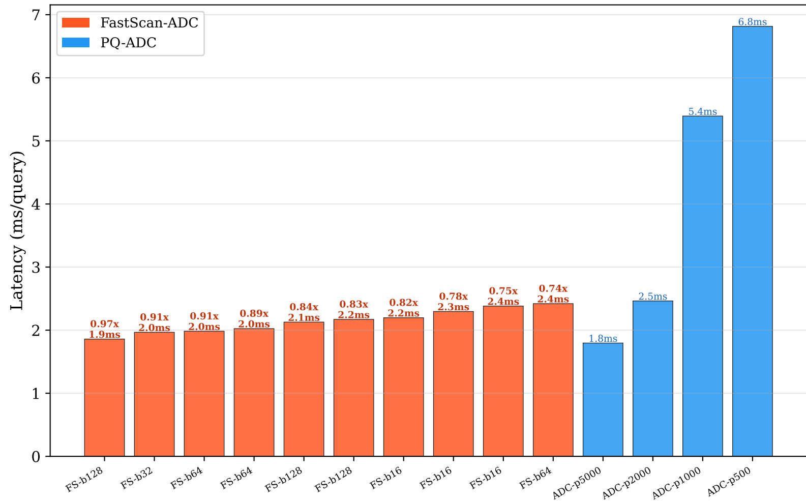
FastScan vs Naive PQ-ADC (M=16, recall=1.0, x86)
