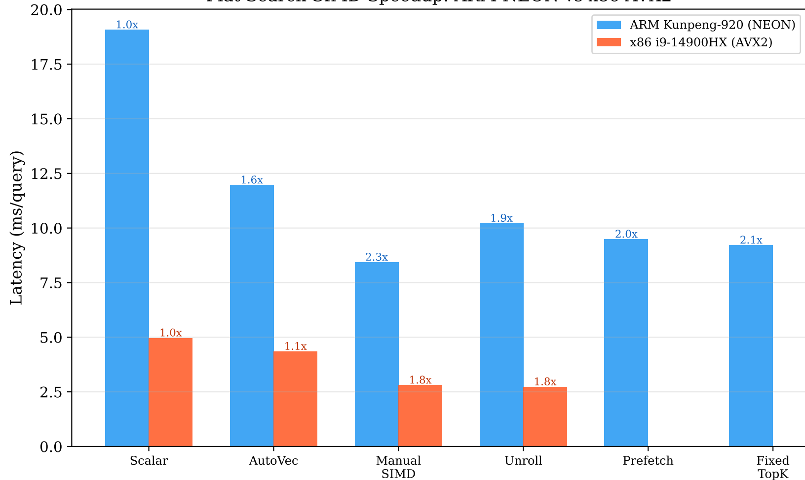
Flat Search SIMD Speedup: ARM NEON vs x86 AVX2
