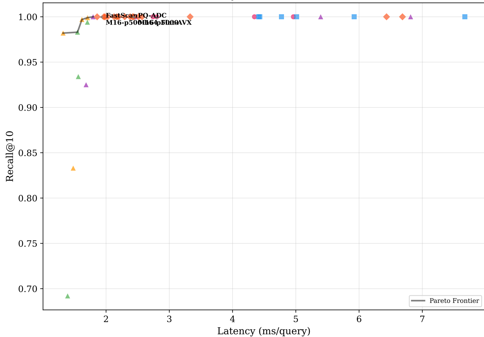
Pareto Frontier: Latency-Recall Trade-off (x86 i9-14900HX)
