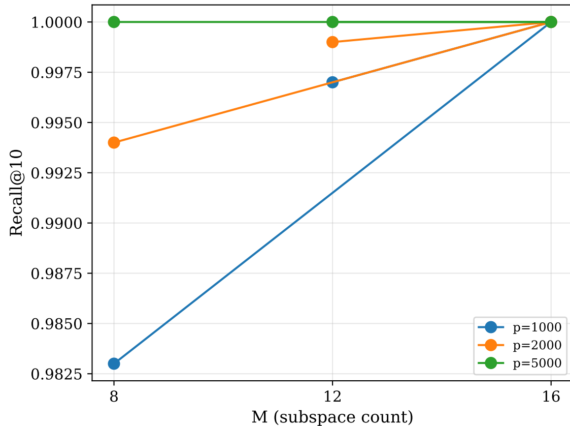
PQ-ADC: M vs Recall
