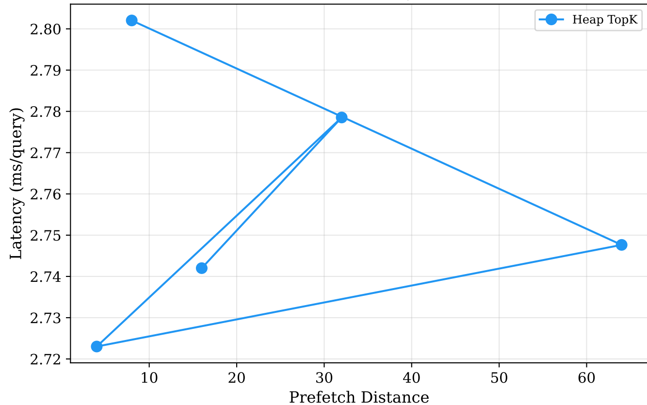
Prefetch Distance Sensitivity (Flat-AVX, x86)
