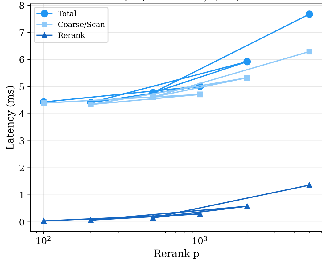
SQ8: p-Sensitivity (x86)
