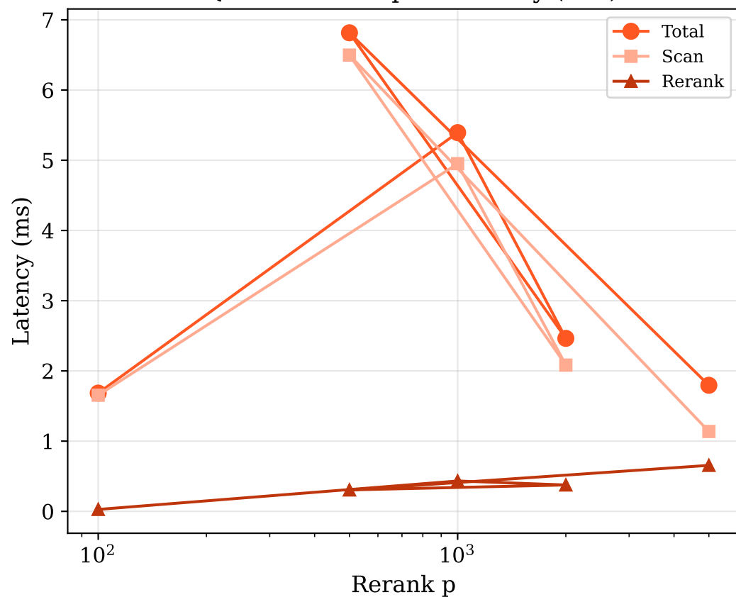
PQ-ADC M=16: p-Sensitivity (x86)
