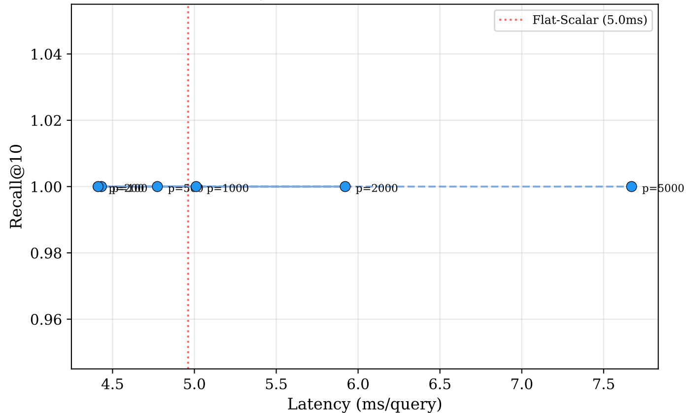
SQ8 Latency-Recall Trade-off (x86 i9-14900HX)
