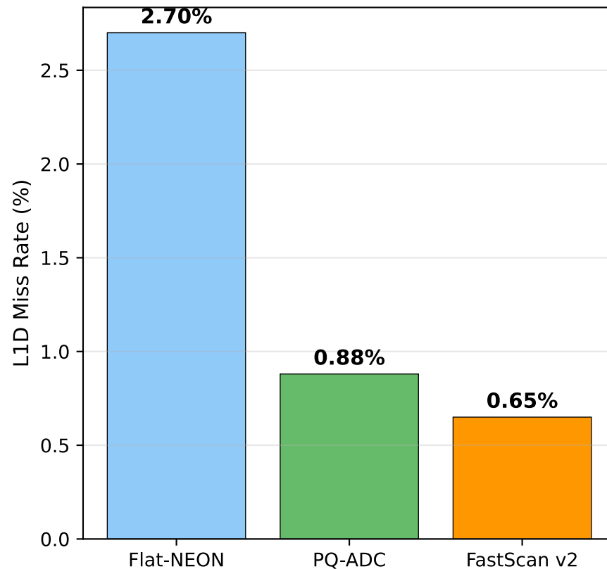
(b) L1 Data Cache Miss
