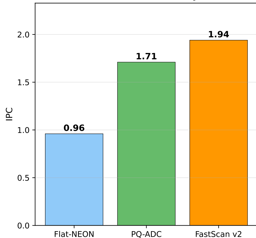
(a) Instructions Per Cycle
