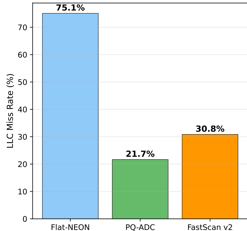
(c) Last-Level Cache Miss
