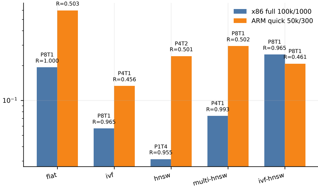
Best algorithm-family latency by platform scale
