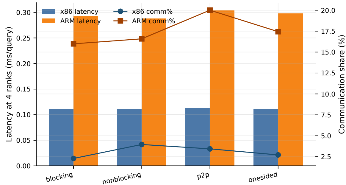
Communication mode comparison at 4 ranks
