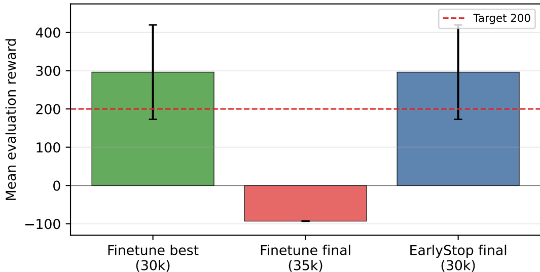
Policy degradation and early stopping
