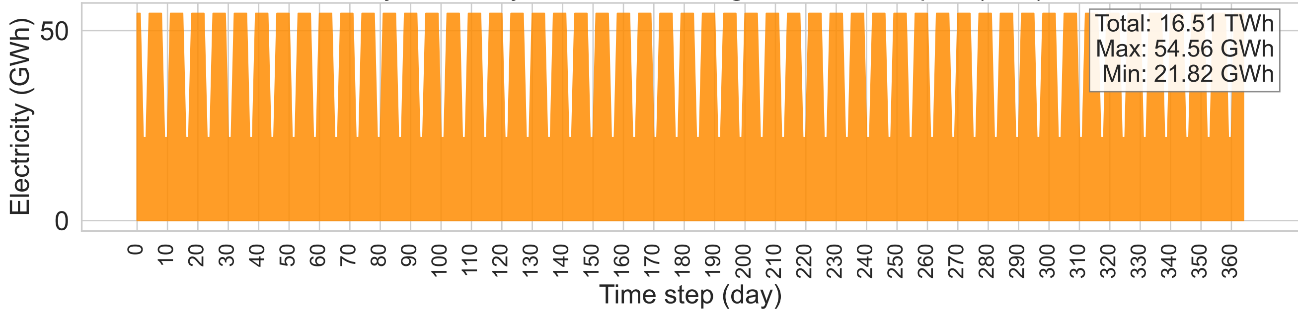
Daily Electricity Demand from Light Road Transport (EVs)
