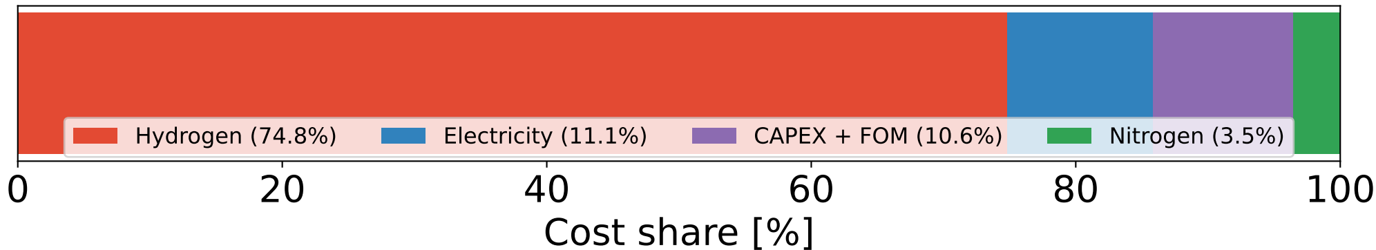
Ammonia ( \text{NH}_3 ) production cost breakdown
