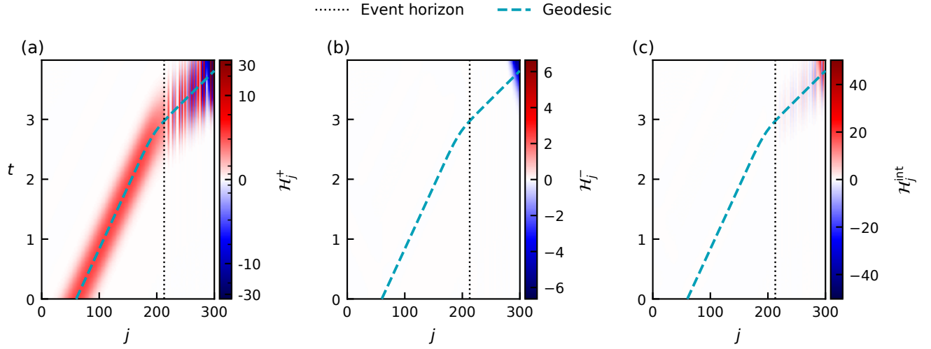
FIG. 4. Wave-packet dynamics in the black-hole geometry for p = 1 . The system parameters, horizon positions, and initial conditions are the same as in Fig. 2. The panels show the branch-resolved energy density \delta\mathcal{E}_{j,s}(t) corresponding to the initially prepared component. Black dotted lines indicate the horizon, and cyan dashed curves show the continuum null trajectories obtained from Eq. (24). Short-wavelength modulations become pronounced in the black-hole interior.
