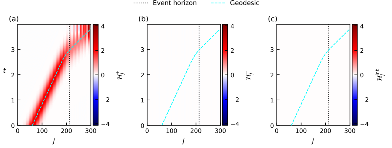
FIG. 2. Wave-packet dynamics in the black-hole geometry for p = 0 . The parameters are L = 300 , \ell = 2\pi , A = 0.6 , B = 3 , and C = 0.6 in the profile defined by Eq. (47). The panels show the branch-resolved energy density \delta\mathcal{E}_{j,s}(t) . In (a,b), x_0 = 2\ell/3 , and the horizon is located at x_h/\ell \simeq 0.709 ( j_h \simeq 213 ). Panel (a) shows an a^+ wave packet initialized outside the horizon at j_{\text{ini}} = 60 , whereas panel (b) shows an a^- wave packet initialized outside the horizon at j_{\text{ini}} = 120 . In (c,d), x_0 = \ell/3 , and the horizon is located at x_h/\ell \simeq 0.376 ( j_h \simeq 113 ). Panels (c) and (d) show a^+ and a^- wave packets, respectively, initialized inside the horizon at j_{\text{ini}} = 150 . In all panels, \sigma_{\text{ini}} = 0.05L . Black dotted lines indicate the horizon, and cyan dashed curves show the corresponding continuum null trajectories obtained from Eq. (24).
