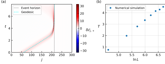
FIG. 8. Wave-packet dynamics in the white-hole geometry for p = 0 . The shift-profile parameters are A = C = -0.6 , B = 3 , x_0 = 2\ell/3 , and \ell = 2\pi . (a) Space-time profile of the vacuum-subtracted branch-resolved energy density \delta\mathcal{E}_{j,+}(t) for L = 300 , j_{\text{ini}} = 0.2L , and \sigma_{\text{ini}} = 0.05L . The black dotted line indicates the white-hole horizon at x_h/\ell \simeq 0.709 ( j_h \simeq 213 ). The packet is compressed as it approaches the horizon but is eventually reflected when its width reaches the lattice scale. (b) Lattice stagnation time T_{\text{lat}} as a function of \ln L for the same continuum profile and initial conditions. Blue dots show the numerical results. Their approximately linear dependence on \ln L is consistent with the cutoff-time scaling derived in the text.
