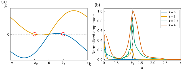
FIG. 6. Finite-momentum structure associated with the modulated wave-packet dynamics for p = 1 . (a) Local dispersion relation at \beta = 1.2 , representative of the deep black-hole interior. Red circles mark the additional zero-energy crossings at \kappa = \pm\kappa_* , where \kappa_* \simeq 1.171 is obtained from Eq. (25). (b) Spatial Fourier spectrum of the wave-packet profile in Fig. 4(a) at t = 0, 3, 3.5 , and 4 , normalized at each time by its maximum value. The black dotted line indicates \kappa_* . The initial peak near \kappa = 0 represents the smooth low-momentum component, whereas a secondary peak develops near the finite-momentum crossing after the packet enters the black-hole interior.
