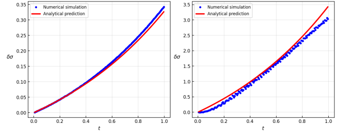
FIG. 7. Extraction of the surface gravity from near-horizon wave-packet broadening. The parameters are L = 500 , A = B = C = 1 , x_0 = \ell/2 , j_{\text{ini}} = 245 , and \sigma_{\text{ini}} = 0.003L . The horizon is located at x_h/\ell = 1/2 ( j_h = 250 ), and the exact surface gravity is \kappa_h = 1 . Blue dots show the numerical change in the standard deviation of the branch-resolved energy density, \delta \sigma_{\mathcal{E}}(t) = \sigma_{\mathcal{E}}(t) - \sigma_{\mathcal{E}}(0) . Red curves show the near-horizon prediction a(e^{\kappa_h t} - 1) with \kappa_h = 1 , where a fixes the vertical scale. The fitted values \kappa_h^{\text{fit}} are obtained separately from fits to a[e^{\kappa_h^{\text{fit}} t} - 1] over t \in [0, 1] . (a) For p = 0 , the relative error in the fitted surface gravity is approximately 0.3%. (b) For p = 1 , the relative error is approximately 9.6%.
