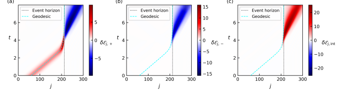
FIG. 9. Wave-packet dynamics in the white-hole geometry for p = 1 . The parameters are L = 300 , A = C = -0.6 , B = 3 , x_0 = 2\ell/3 , j_{\text{ini}} = 0.2L , and \sigma_{\text{ini}} = 0.05L . The white-hole horizon is located at x_h/\ell \simeq 0.709 ( j_h \simeq 213 ). Panels (a)–(c) show the vacuum-subtracted contributions \delta\mathcal{E}_{j,+}(t) , \delta\mathcal{E}_{j,-}(t) , and \delta\mathcal{E}_{j,\text{int}}(t) , respectively. The black dotted line indicates the horizon. Unlike the p = 0 case, finite-spacing mixing between the two components produces mode conversion and partial transmission into the white-hole interior.
