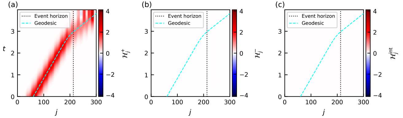
FIG. 2. Wave-packet dynamics in the black-hole geometry for p = 0 . The parameters are L = 300 , \ell = 2\pi , A = 0.6 , B = 3 , and C = 0.6 in the profile defined by Eq. (47). The panels show the branch-resolved energy density \delta\mathcal{E}_{j,s}(t) . In (a,b), x_0 = 2\ell/3 , and the horizon is located at x_h/\ell \simeq 0.709 ( j_h \simeq 213 ). Panel (a) shows an a^+ wave packet initialized outside the horizon at j_{\text{ini}} = 60 , whereas panel (b) shows an a^- wave packet initialized outside the horizon at j_{\text{ini}} = 120 . In (c,d), x_0 = \ell/3 , and the horizon is located at x_h/\ell \simeq 0.376 ( j_h \simeq 113 ). Panels (c) and (d) show a^+ and a^- wave packets, respectively, initialized inside the horizon at j_{\text{ini}} = 150 . In all panels, \sigma_{\text{ini}} = 0.05L . Black dotted lines indicate the horizon, and cyan dashed curves show the corresponding continuum null trajectories obtained from Eq. (24).
