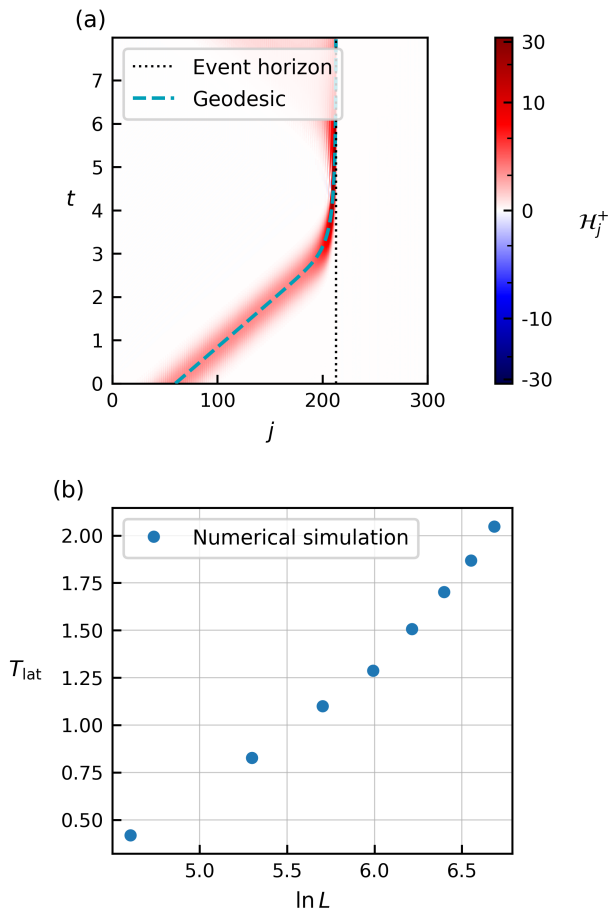
FIG. 8. Wave-packet dynamics in the white-hole geometry for p = 0 . The shift-profile parameters are A = C = -0.6 , B = 3 , x_0 = 2\ell/3 , and \ell = 2\pi . (a) Space-time profile of the vacuum-subtracted branch-resolved energy density \delta\mathcal{E}_{j,+}(t) for L = 300 , j_{\text{ini}} = 0.2L , and \sigma_{\text{ini}} = 0.05L . The black dotted line indicates the white-hole horizon at x_h/\ell \simeq 0.709 ( j_h \simeq 213 ). The packet is compressed as it approaches the horizon but is eventually reflected when its width reaches the lattice scale. (b) Lattice stagnation time T_{\text{lat}} as a function of \ln L for L = 100, 200, \dots, 800 , using the same continuum profile and initial conditions. Blue dots show the numerical results. Their approximately linear dependence on \ln L is consistent with the cutoff-time scaling derived in the text.
