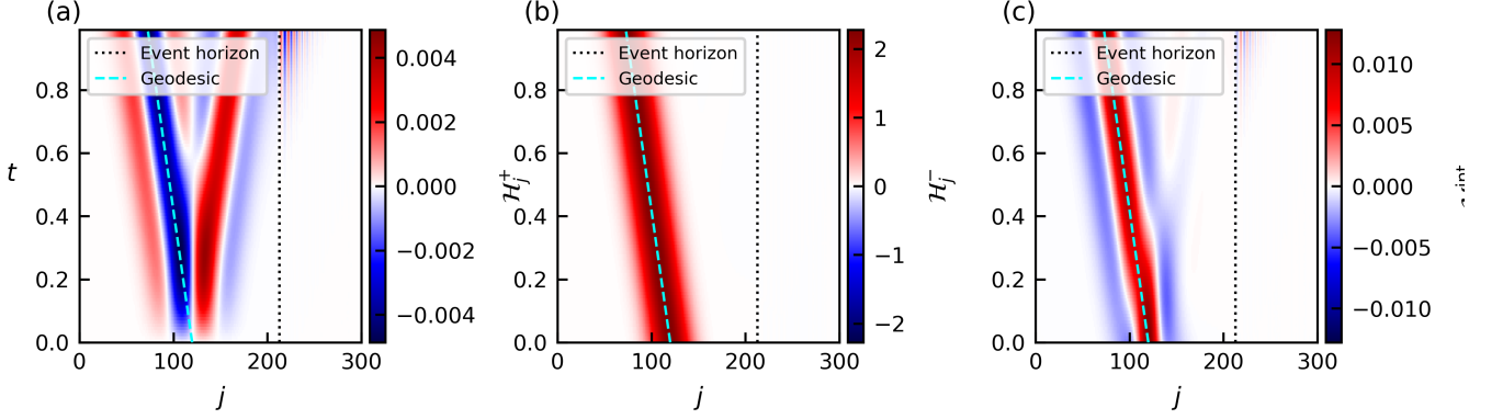
FIG. 5. Wave-packet dynamics in the black-hole geometry for p = 1 for an initially prepared a^- wave packet outside the horizon. The parameters and horizon position are the same as in Fig. 4, except that the packet is initialized at j_{\text{ini}} = 120 . Panels (a)–(c) show the vacuum-subtracted contributions \delta\mathcal{E}_{j,+}(t) , \delta\mathcal{E}_{j,-}(t) , and \delta\mathcal{E}_{j,\text{int}}^{(-)}(t) , respectively. Black dotted lines indicate the horizon, and cyan dashed curves show the corresponding continuum null trajectories obtained from Eq. (24).
