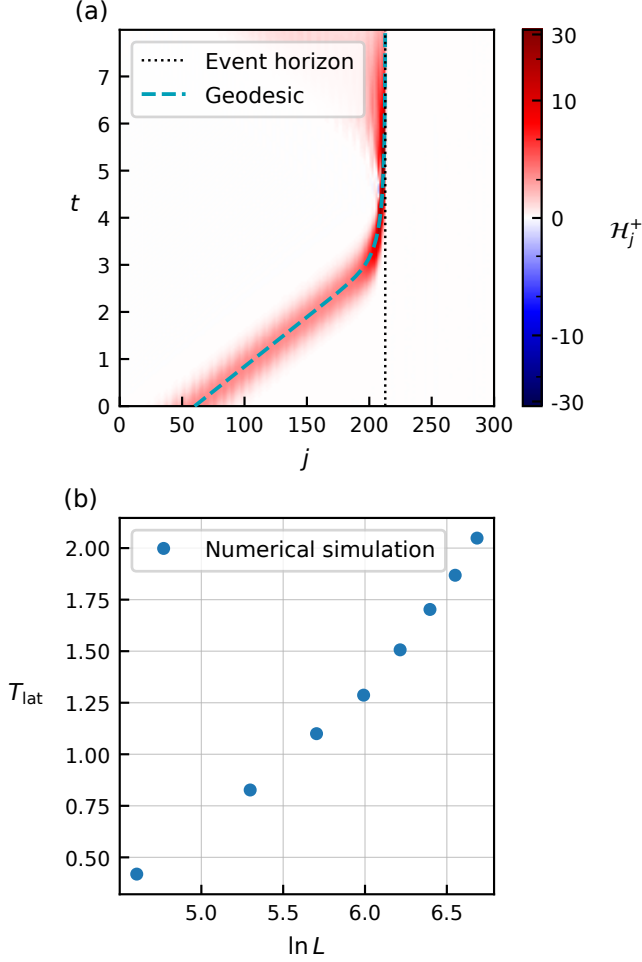
FIG. 8. Wave packet dynamics in the white-hole geometry for p = 0 . (a) Space-time diagram of \mathcal{H}_j^+ for L = 300 , j_0 = 0.2L , and \sigma = 0.05L , with \beta profile parameters A = C = -0.6 , B = 3 , and x_0 = 2\ell/3 (white-hole horizon at j_h \approx 213 ). The symmetric asinh color mapping in Eq. (50) is used with \mathcal{H}_0 = 3 . The wave packet is compressed toward the white-hole horizon (black dotted line) and eventually reflected due to finite lattice resolution. (b) Lattice stagnation time T_{\text{lat}} versus \ln L for various system sizes, using A = C = -0.6 , B = 3 , x_0 = 2\ell/3 , j_0 = 0.2L , and \sigma = 0.05L . Blue dots show numerical simulation results; their approximately linear dependence on \ln L is consistent with the logarithmic scaling of Eq. (52).
