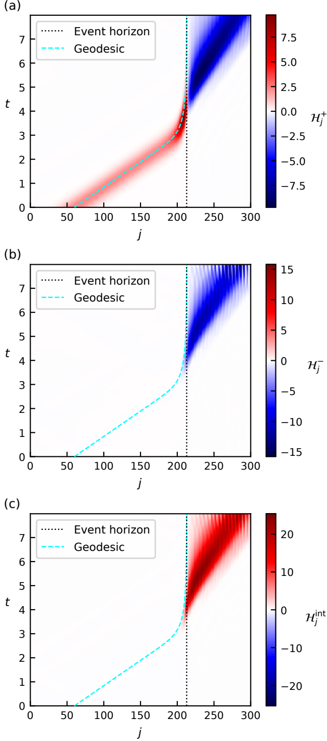
FIG. 9. White-hole dynamics for p = 1 ( L = 300 , j_0 = 0.2L , \sigma = 0.05L , with the same \beta profile as Fig. 8(a), A = C = -0.6 , B = 3 , x_0 = 2\ell/3 , and j_h \approx 213 ). (a) Space-time diagram of \mathcal{H}_j^+ . (b) Space-time diagram of \mathcal{H}_j^- . (c) Space-time diagram of the interaction contribution \mathcal{H}_j^{\text{int}} . Unlike the p = 0 case, the coupling between the right- and left-moving components allows partial transmission across the white-hole horizon (black dotted line).
