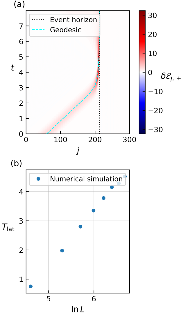
FIG. 6. Wave packet dynamics in the white-hole geometry for p = 0 . (a) Space-time diagram of the vacuum-subtracted energy density \delta\mathcal{E}_{j,+} [Eq. (44)] for L = 300 , j_0 = 0.2L , and \sigma = 0.05L , with \beta profile parameters A = C = -0.6 , B = 3 , and x_0 = 2\ell/3 (white-hole horizon at j_h \approx 213 ). The wave packet is compressed toward the white-hole horizon (black dotted line) and eventually reflected due to finite lattice resolution. (b) Lattice stagnation time T_{\text{lat}} versus \ln L for various system sizes, using A = C = -0.6 , B = 3 , x_0 = 2\ell/3 , j_0 = 0.2L , and \sigma = 0.05L . Blue dots show numerical simulation results; their approximately linear dependence on \ln L is consistent with the logarithmic scaling of Eq. (52).
