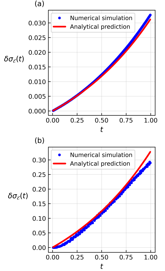
FIG. 5. Extraction of surface gravity from wave-packet broadening ( L = 500 , A = B = C = 1 , x_0 = \ell/2 , j_0 = 245 , \sigma = 0.003L , with the fit performed over t \in [0, 1] ). Blue dots show the numerical energy-density-weighted width \delta\sigma_\epsilon(t) defined in Eq. (45), and red curves show the analytical near-horizon scaling a(e^{\kappa t} - 1) with \kappa = 1 ; the prefactor a fixes the vertical scale. The fitted growth rates are obtained separately from a(e^{\kappa_{\text{fit}} t} - 1) . (a) Result for p = 0 , with |\kappa_{\text{fit}} - \kappa|/\kappa \approx 3.3\% . (b) Result for p = 1 , with |\kappa_{\text{fit}} - \kappa|/\kappa \approx 4.9\% due to simultaneous wave packet dispersion. These percentages quantify the error in the fitted surface gravity, not the pointwise deviation of the red analytical curves.
