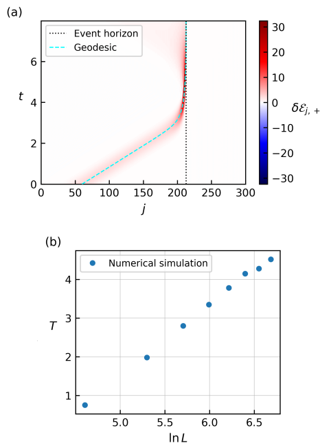
FIG. 8. Wave-packet dynamics in the white-hole geometry for p = 0 . The shift-profile parameters are A = C = -0.6 , B = 3 , x_0 = 2\ell/3 , and \ell = 2\pi . (a) Space-time profile of the vacuum-subtracted branch-resolved energy density \delta\mathcal{E}_{j,+}(t) for L = 300 , j_{\text{ini}} = 0.2L , and \sigma_{\text{ini}} = 0.05L . The black dotted line indicates the white-hole horizon at x_h/\ell \simeq 0.709 ( j_h \simeq 213 ). The packet is compressed as it approaches the horizon but is eventually reflected when its width reaches the lattice scale. (b) Lattice stagnation time T_{\text{lat}} as a function of \ln L for L = 100, 200, \dots, 800 , using the same continuum profile and initial conditions. Blue dots show the numerical results. Their approximately linear dependence on \ln L is consistent with the cutoff-time scaling derived in the text.
